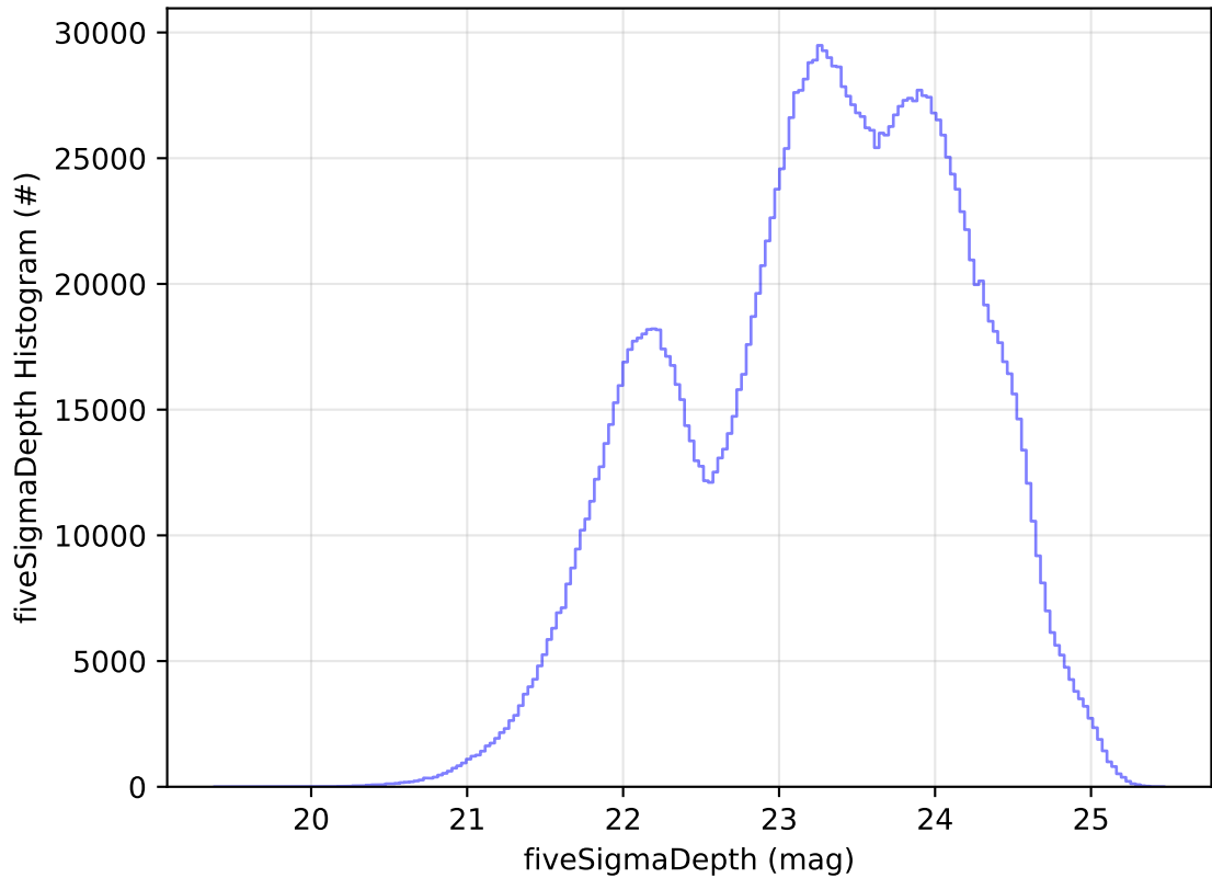
ddf_acor_sf15_lsf30_lsr20_v3.4_10yrs All sky all bands: fiveSigmaDepth Histogram
