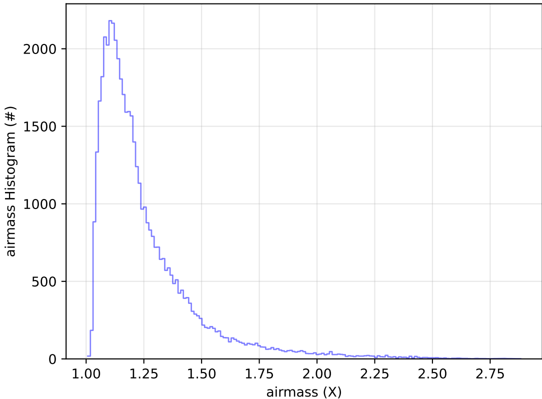
ddf_acor_sf15_lsf30_lsr20_v3.4_10yrs Yr 1 y band: airmass Histogram
