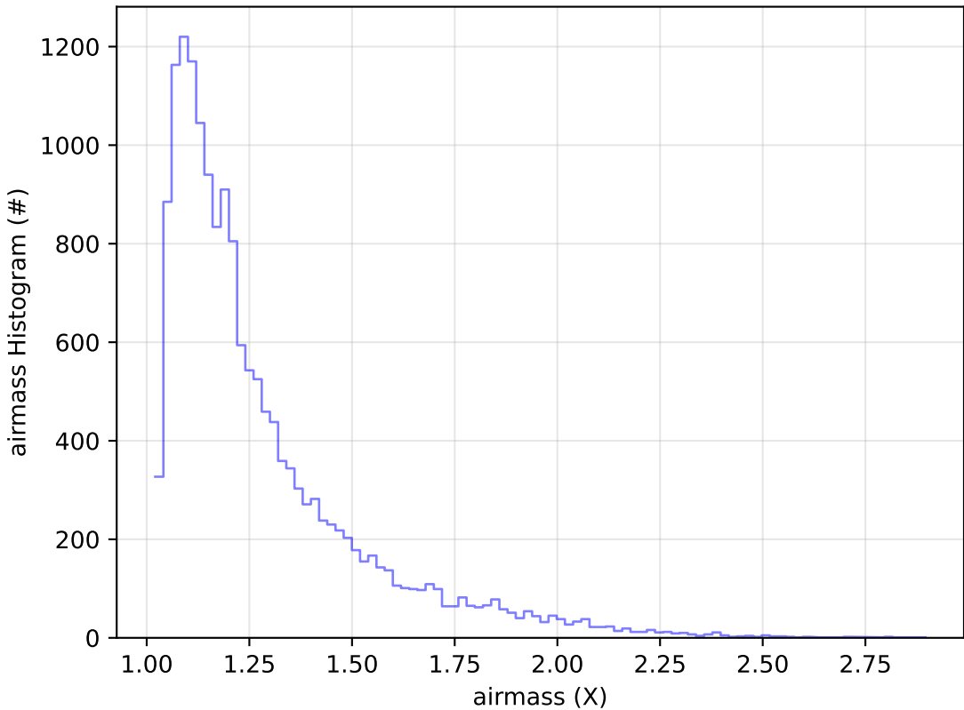
ddf_acor_sf15_ls30_lsr20_v3.4_10yrs Yr 1 u band: airmass Histogram
