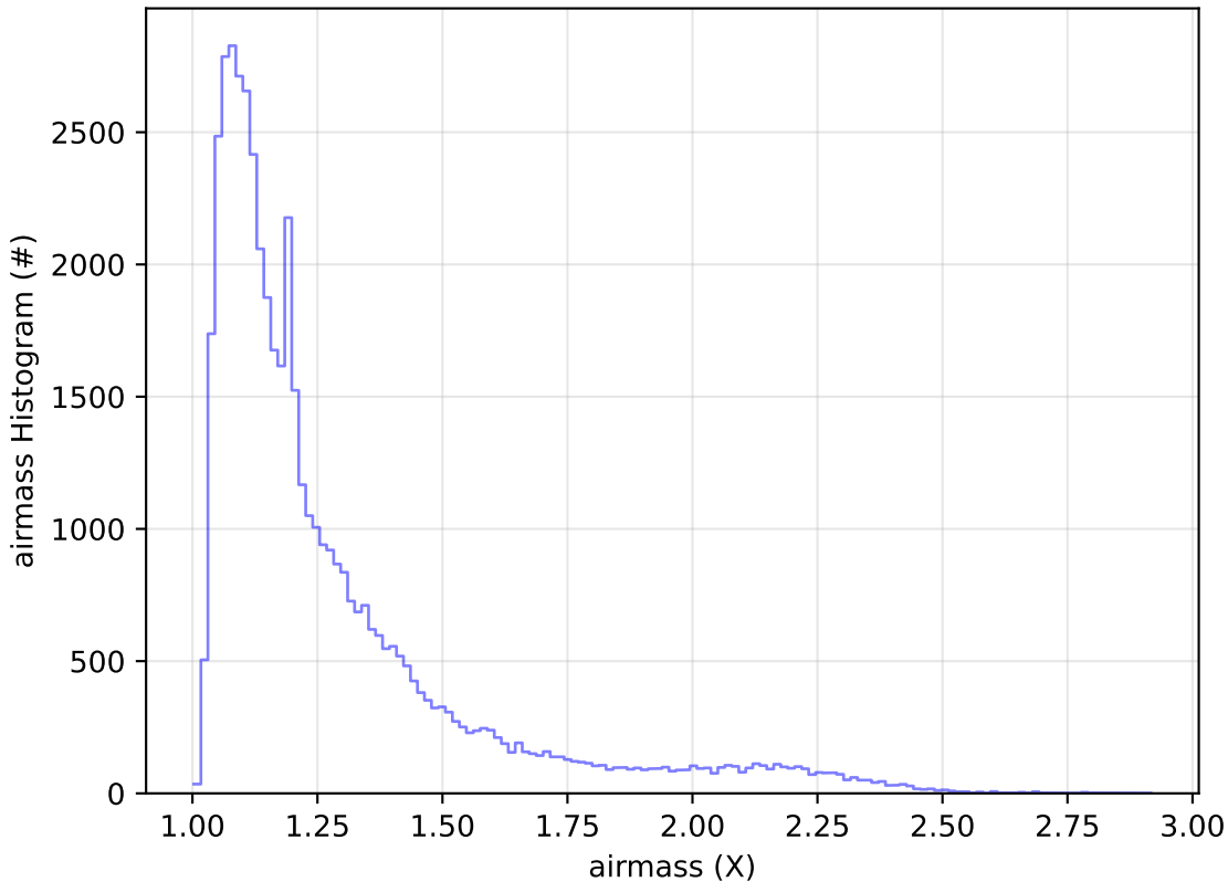
ddf_acor_sf15_lsf30_lsr20_v3.4_10yrs Yr 1 r band: airmass Histogram
