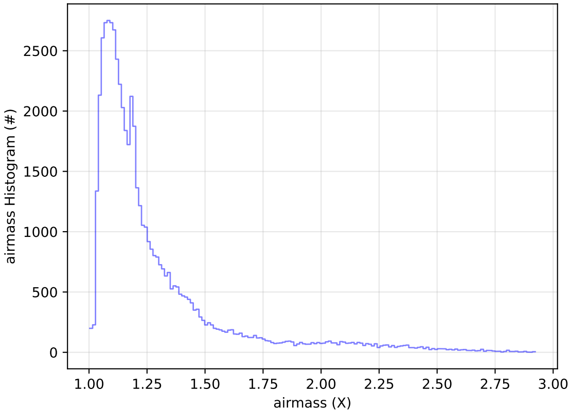
ddf_acor_sf15_lsf30_lsr20_v3.4_10yrs Yr 1 i band: airmass Histogram
