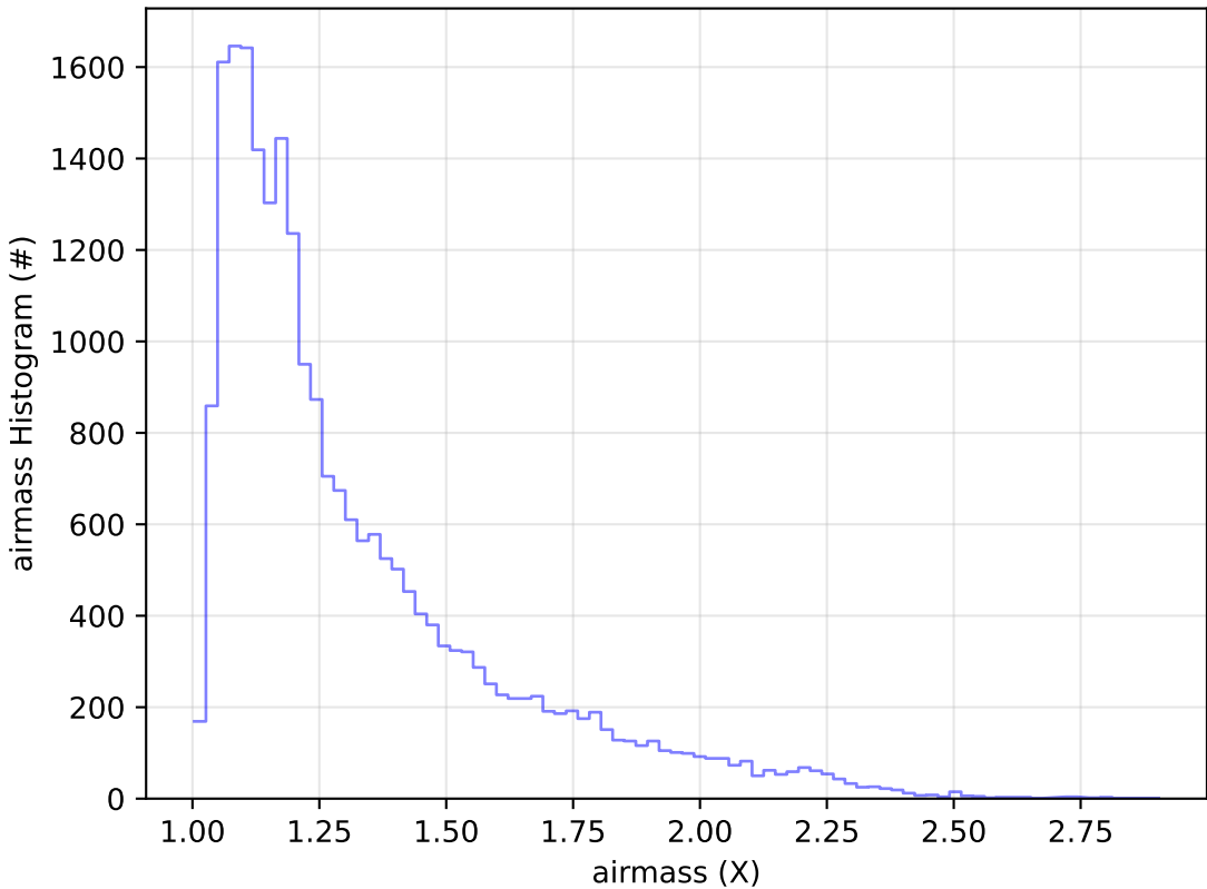
ddf_acor_sf15_lsf30_lsr20_v3.4_10yrs Yr 1 g band: airmass Histogram
