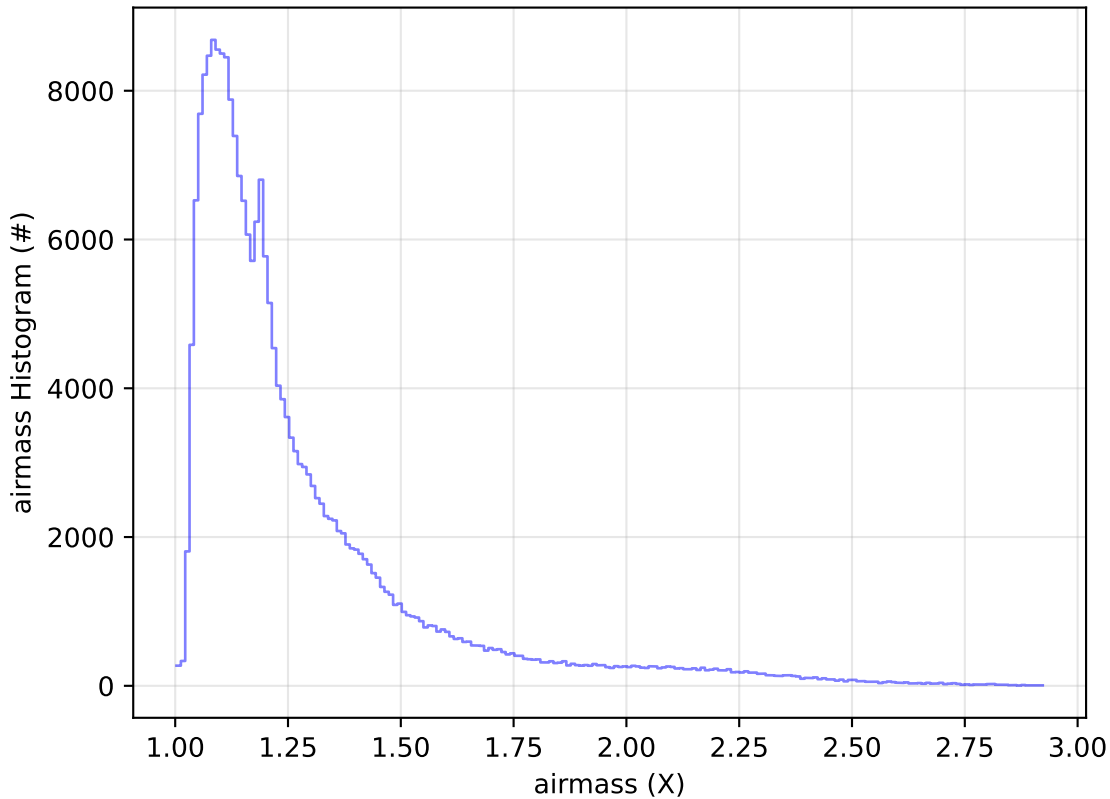
ddf_acor_sf15_lsf30_lsr20_v3.4_10yrs Yr 1 all bands: airmass Histogram
