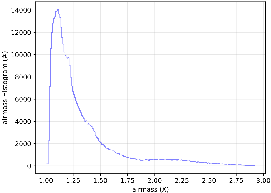
ddf_acor_sf15_lsf30_lsr20_v3.4_10yrs WFD z band: airmass Histogram
