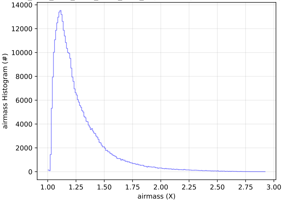
ddf_acor_sf15_lsf30_lsr20_v3.4_10yrs WFD y band: airmass Histogram
