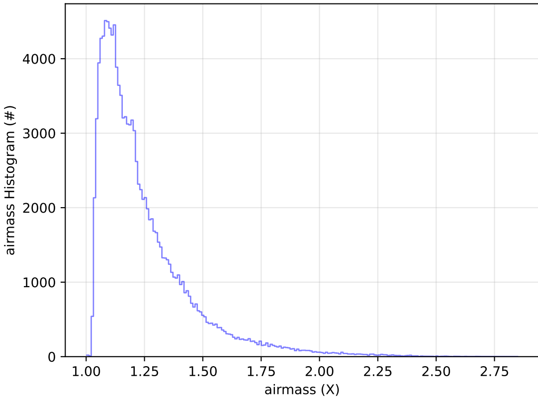
ddf_acor_sf15_lsf30_lsr20_v3.4_10yrs WFD u band: airmass Histogram
