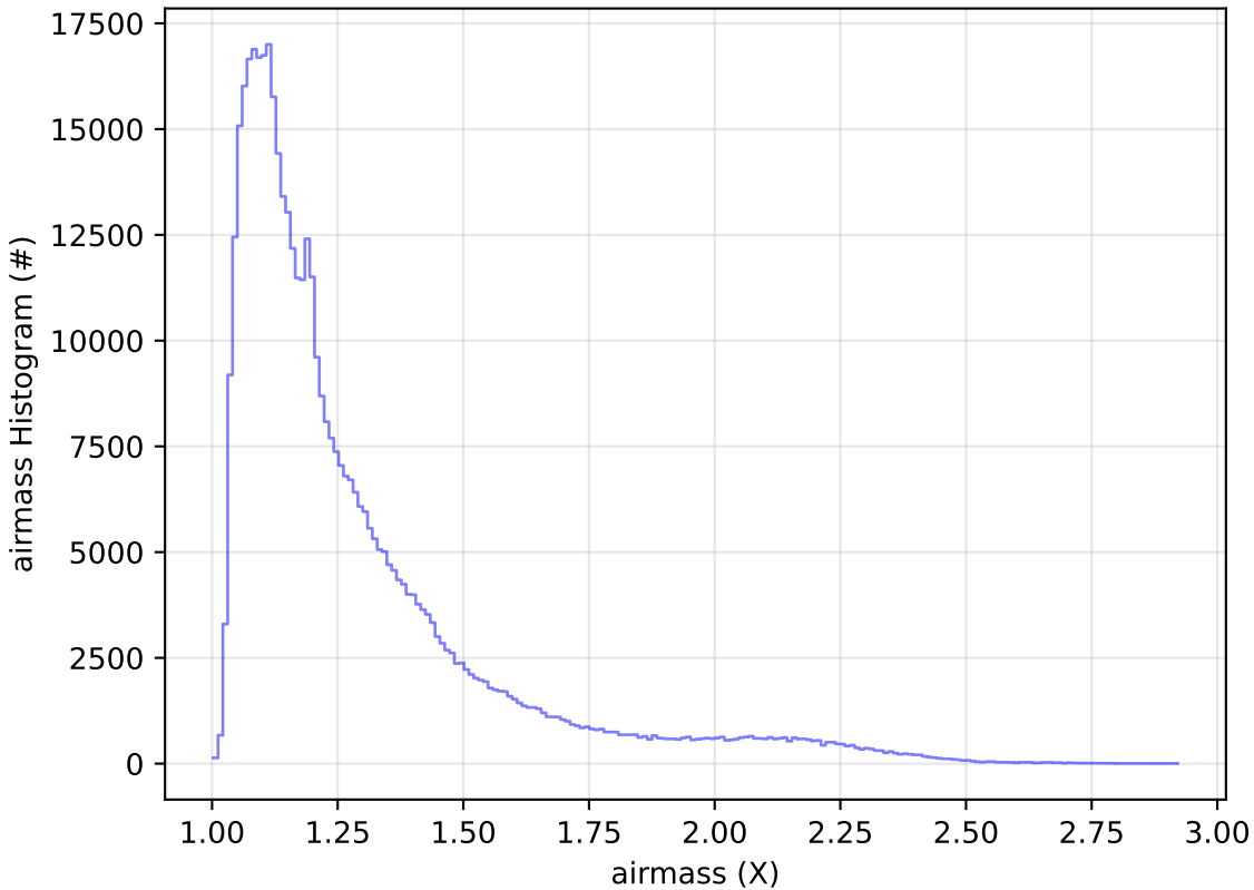
ddf_acor_sf15_lsf30_lsr20_v3.4_10yrs WFD r band: airmass Histogram
