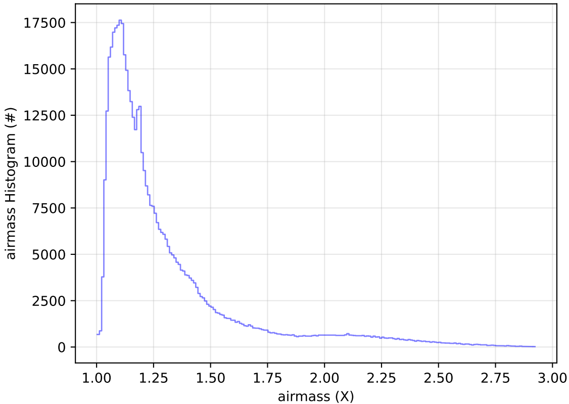
ddf_acor_sf15_lsf30_lsr20_v3.4_10yrs WFD i band: airmass Histogram
