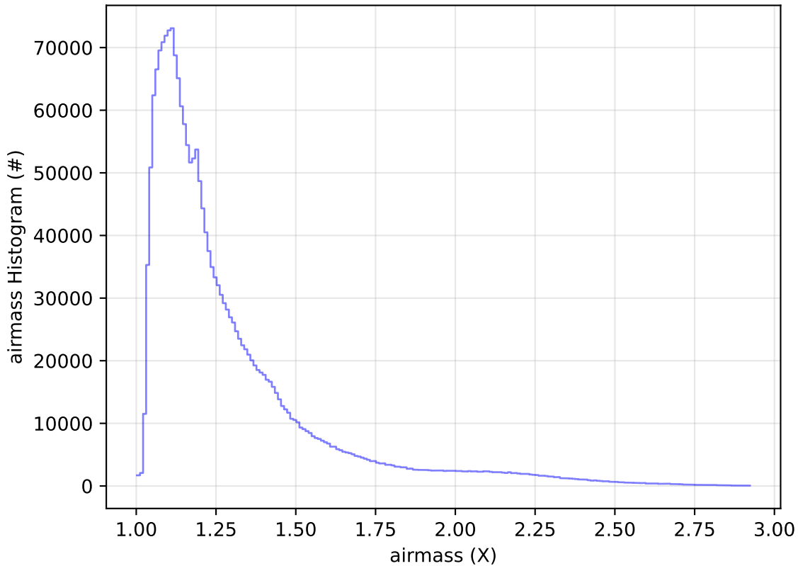
ddf_acor_sf15_lsf30_lsr20_v3.4_10yrs WFD all bands: airmass Histogram
