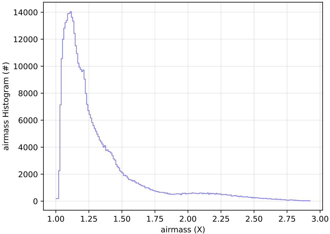
ddf_acor_sf15_lsf30_lsr20_v3.4_10yrs All sky z band: airmass Histogram
