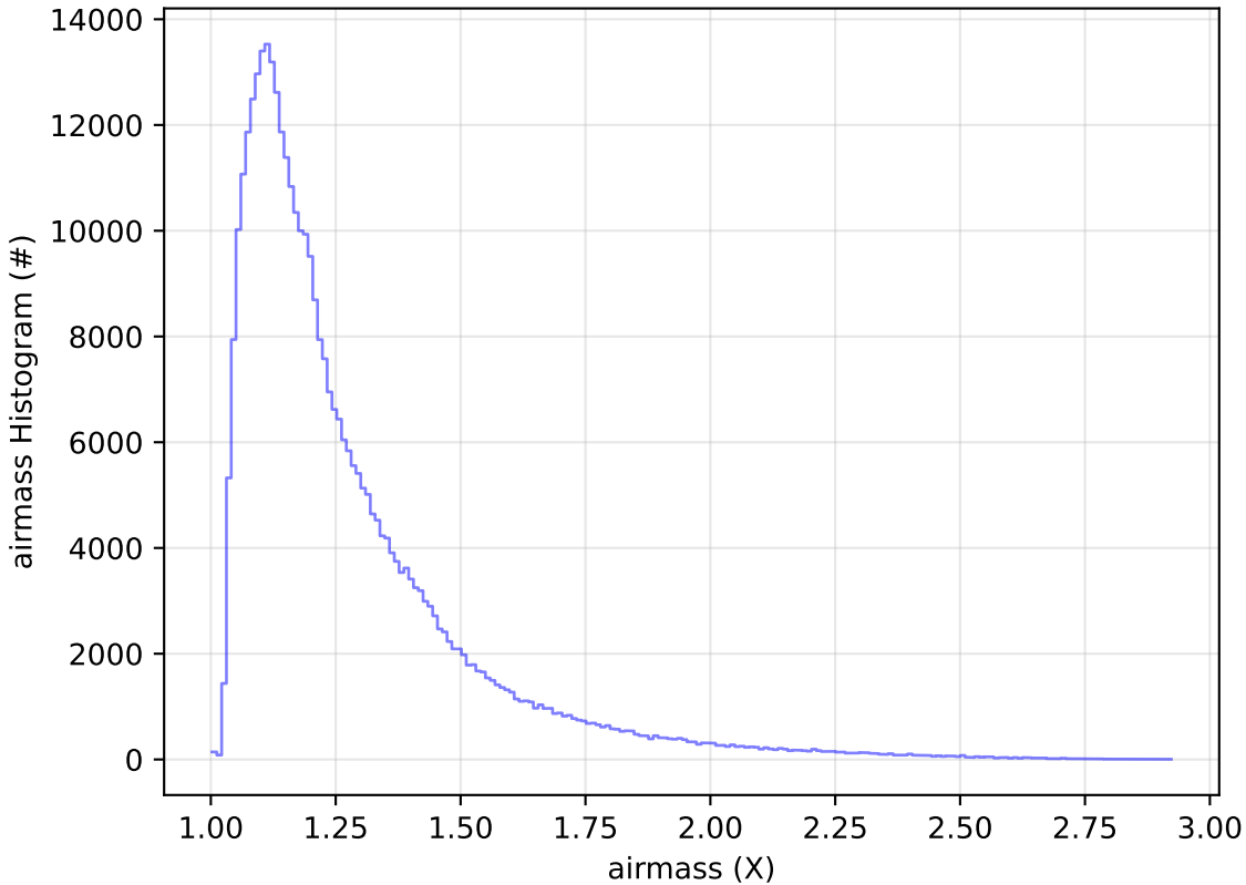
ddf_acor_sf15_lsf30_lsr20_v3.4_10yrs All sky y band: airmass Histogram
