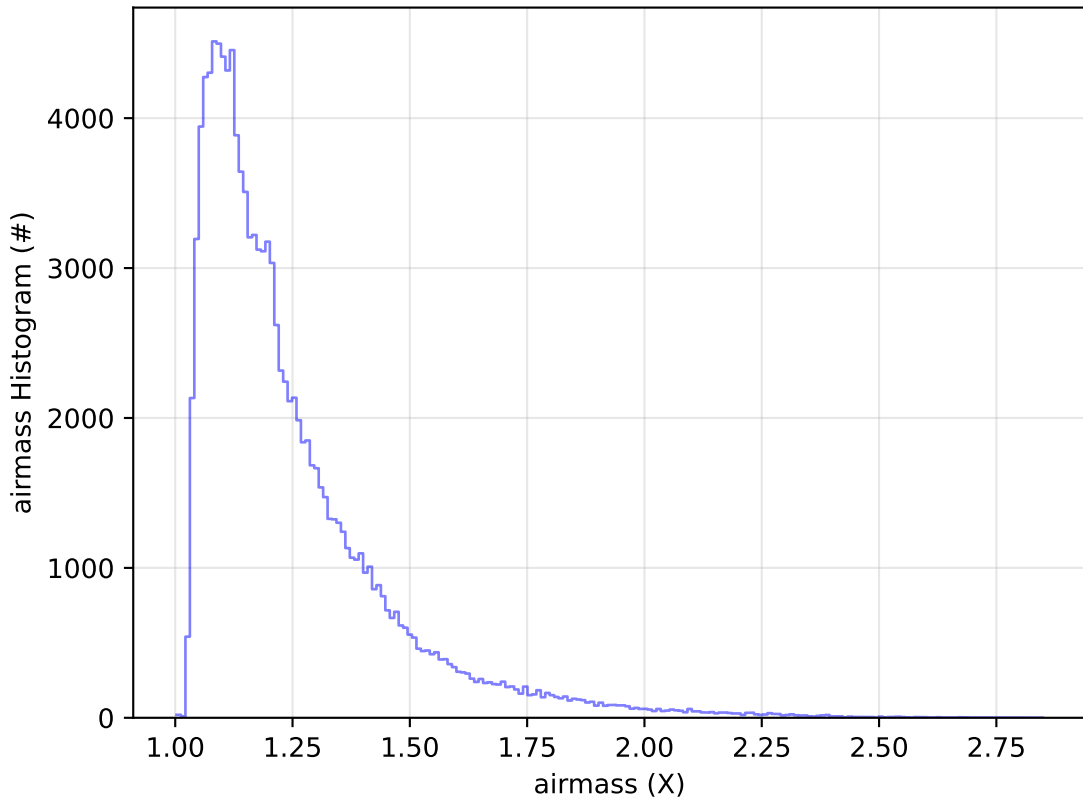
ddf_acor_sf15_lsf30_lsr20_v3.4_10yrs All sky u band: airmass Histogram
