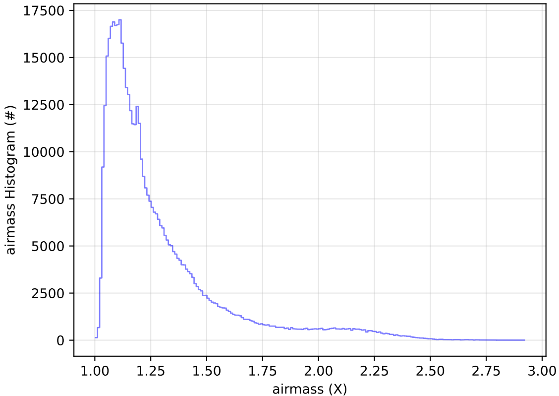
ddf_acor_sf15_lsf30_lsr20_v3.4_10yrs All sky r band: airmass Histogram
