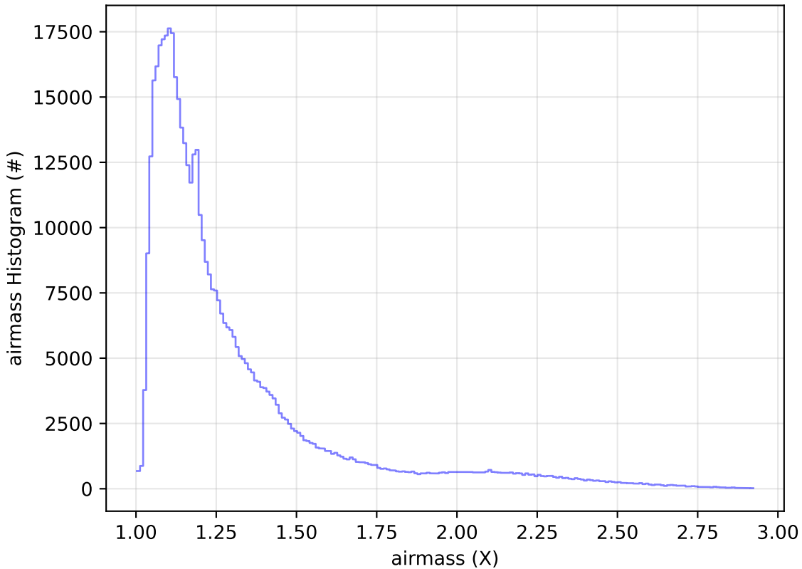
ddf_acor_sf15_lsf30_lsr20_v3.4_10yrs All sky i band: airmass Histogram
