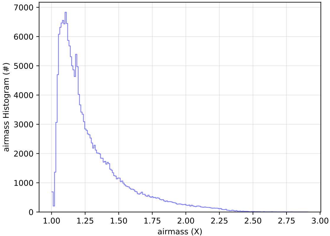
ddf_acor_sf15_lsf30_lsr20_v3.4_10yrs All sky g band: airmass Histogram
