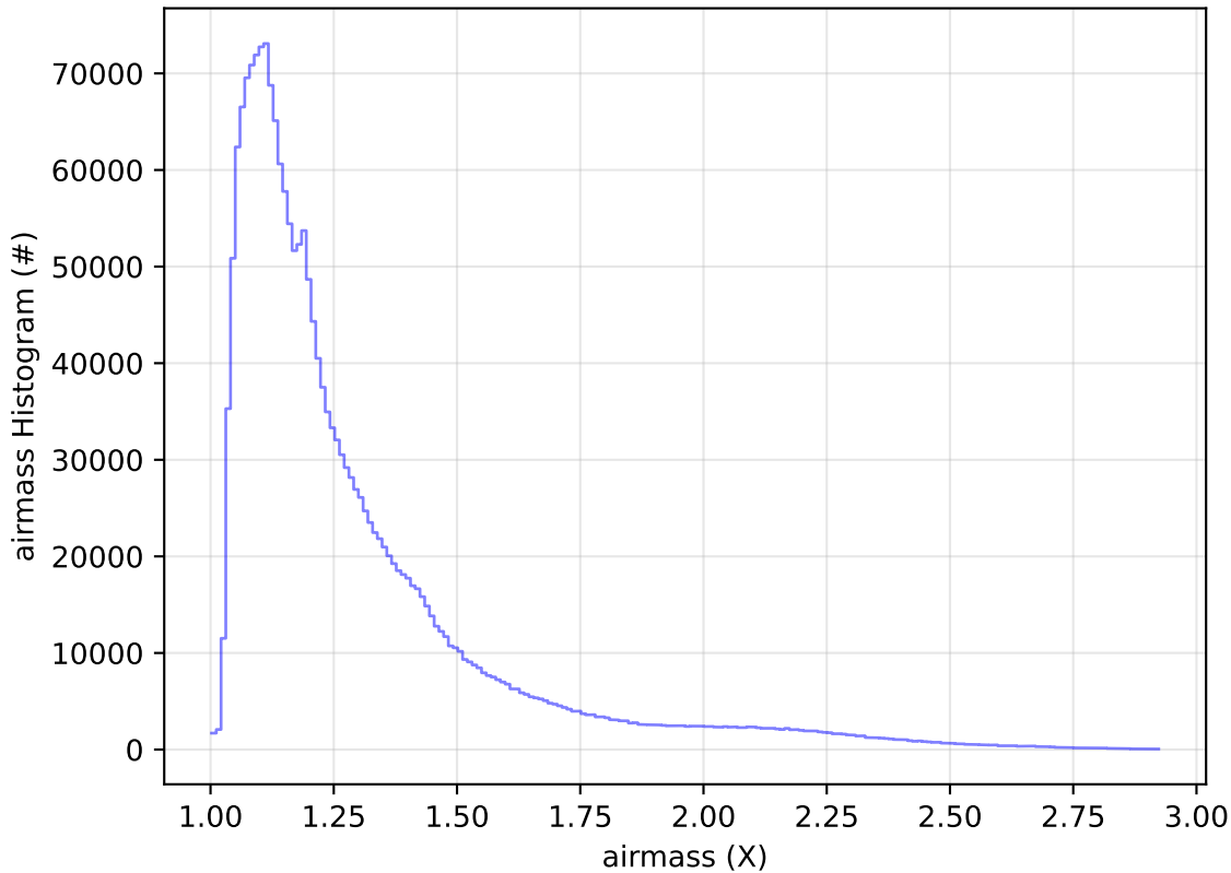
ddf_acor_sf15_lsf30_lsr20_v3.4_10yrs All sky all bands: airmass Histogram
