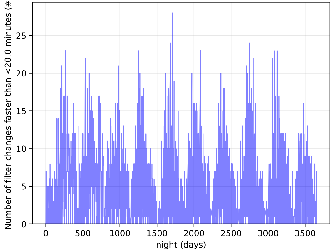
ddf_acor_sf15_Isf30_Isr20_v3.4_10yrs Per Night: Number of filter changes faster than <20.0 minutes
