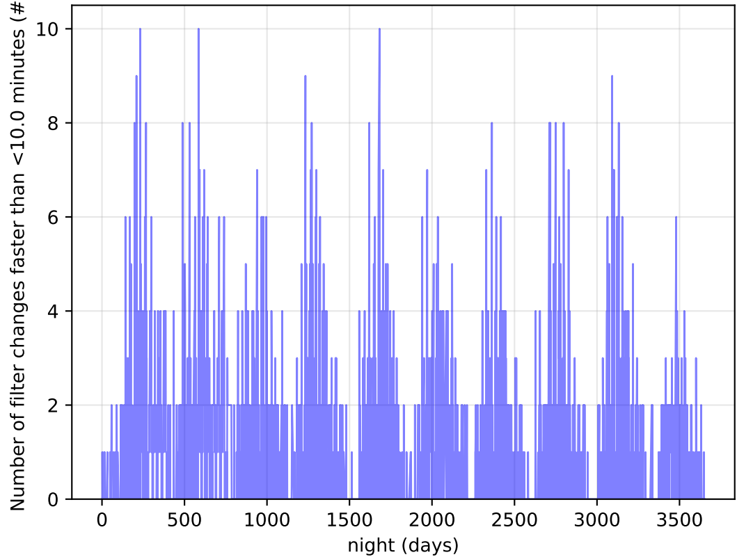
ddf_acor_sf15_Isf30_Isr20_v3.4_10yrs Per Night: Number of filter changes faster than <10.0 minutes
