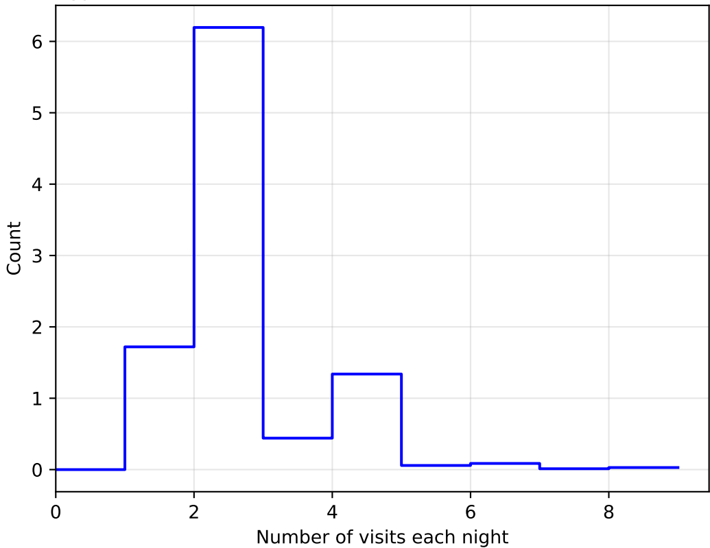
ddf_acor_sf15_lsf30_lsr20_v3.4_10yrs All sky: NVisitsPerNight 1e6
