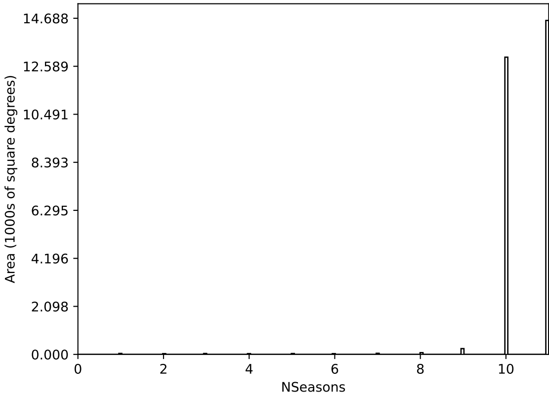
ddf_acor_sf15_lsf30_lsr20_v3.4_10yrs All sky all bands: NSeasons
