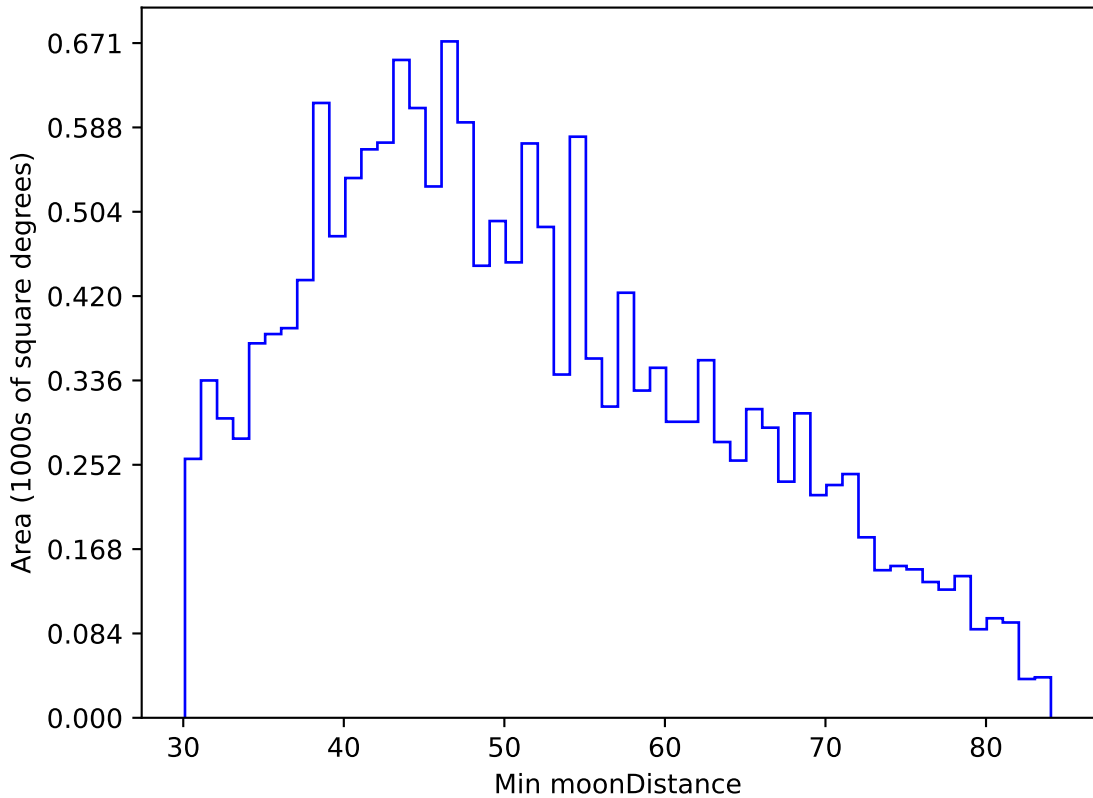
ddf_acor_sf15_lsf30_lsr20_v3.4_10yrs WFD u band: Min moonDistance
