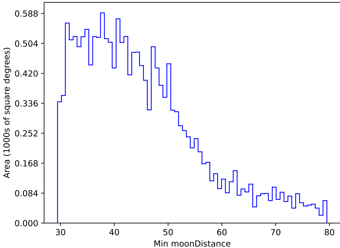
ddf_acor_sf15_lsf30_lsr20_v3.4_10yrs WFD g band: Min moonDistance
