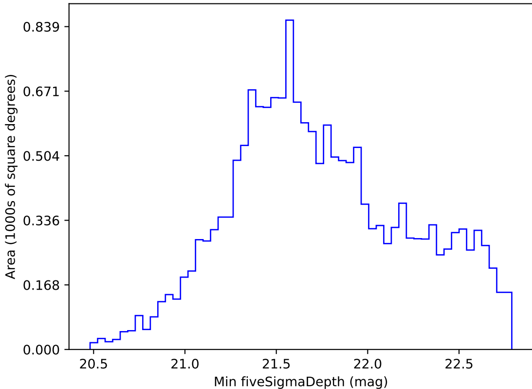
ddf_acor_sf15_lsf30_lsr20_v3.4_10yrs WFD i band: Min fiveSigmaDepth
