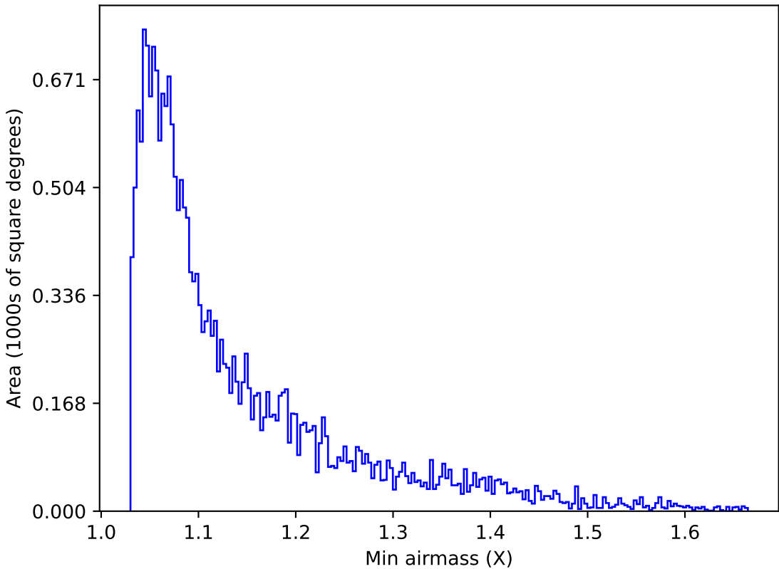
ddf_acor_sf15_lsf30_lsr20_v3.4_10yrs Yr 1 u band: Min airmass
