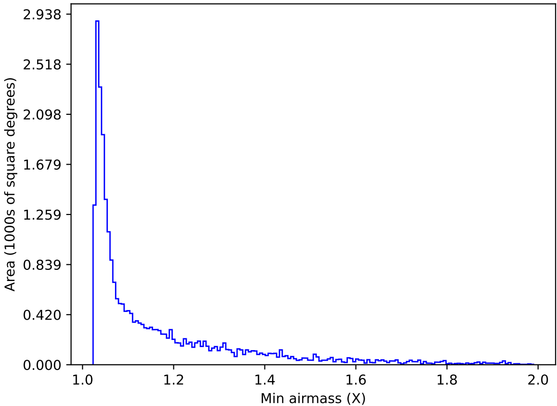
ddf_acor_sf15_lsf30_lsr20_v3.4_10yrs Yr 1 r band: Min airmass
