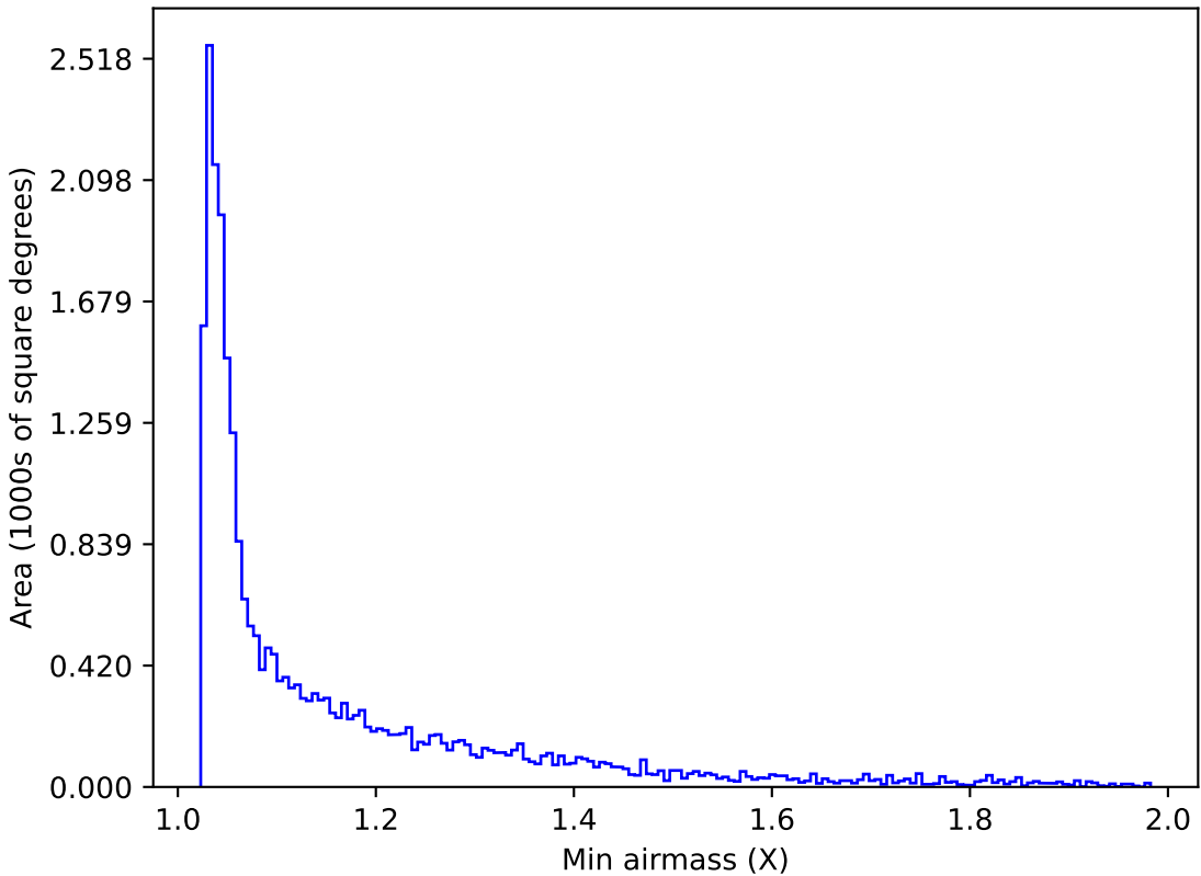
ddf_acor_sf15_lsf30_lsr20_v3.4_10yrs Yr 1 i band: Min airmass
