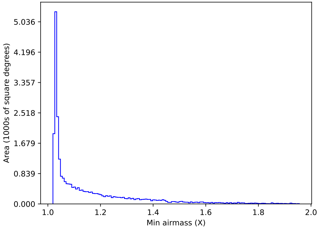
ddf_acor_sf15_lsf30_lsr20_v3.4_10yrs Yr 1 all bands: Min airmass
