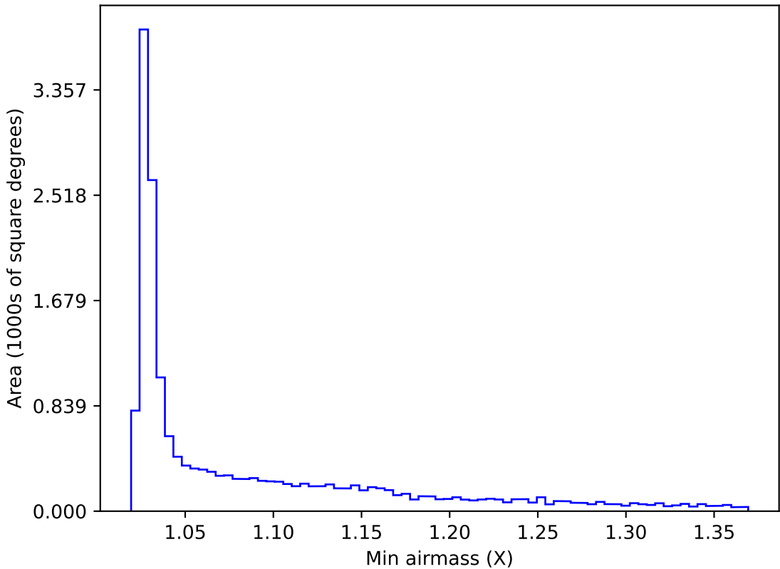
ddf_acor_sf15_lsf30_lsr20_v3.4_10yrs WFD z band: Min airmass
