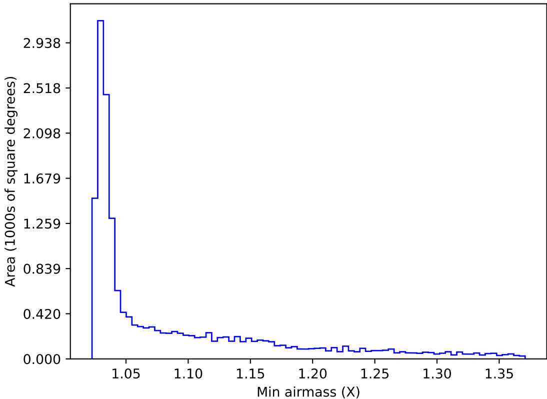
ddf_acor_sf15_lsf30_lsr20_v3.4_10yrs WFD y band: Min airmass
