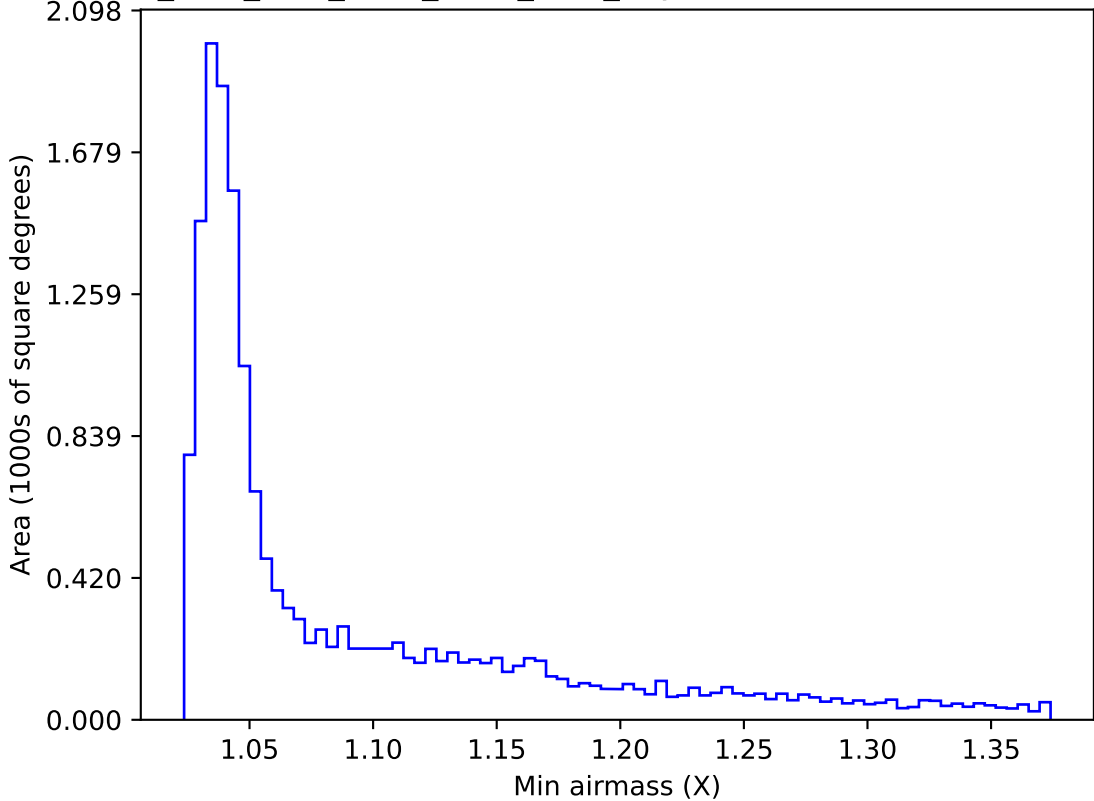
ddf_acor_sf15_lsf30_lsr20_v3.4_10yrs WFD u band: Min airmass
