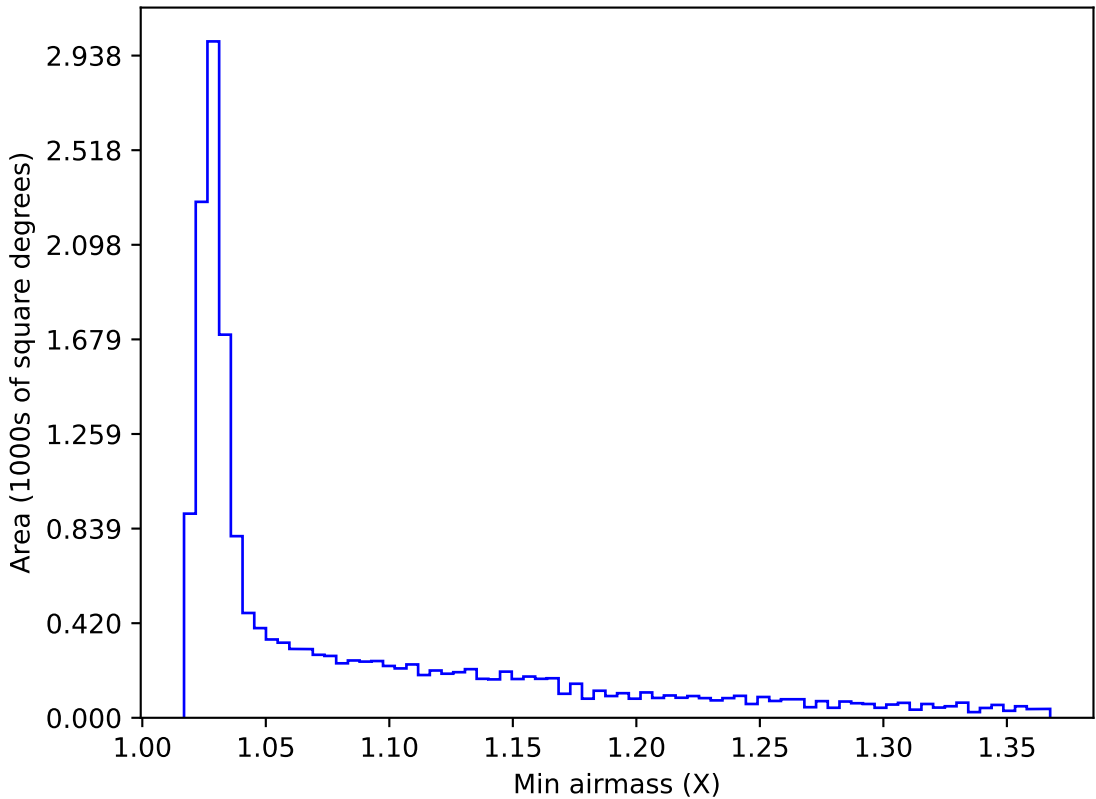
ddf_acor_sf15_lsf30_lsr20_v3.4_10yrs WFD r band: Min airmass
