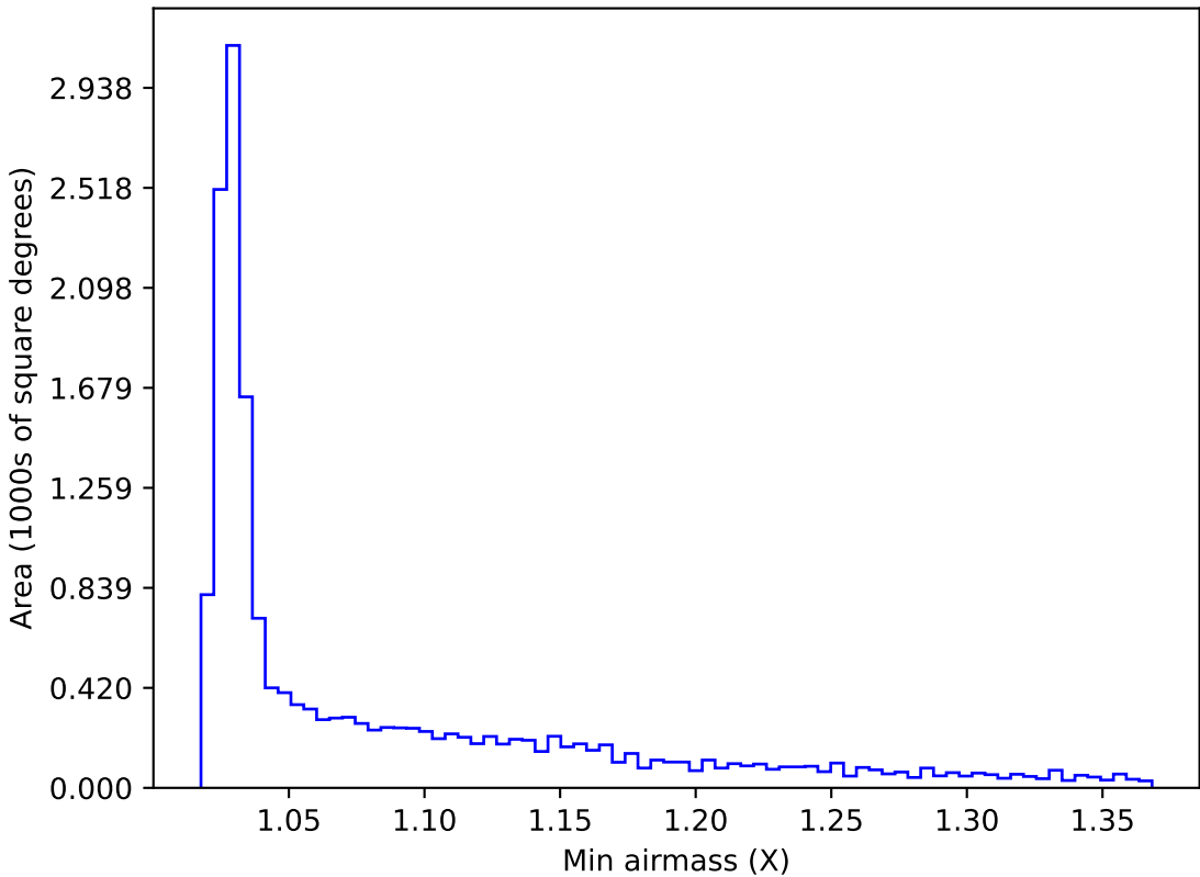
ddf_acor_sf15_lsf30_lsr20_v3.4_10yrs WFD i band: Min airmass
