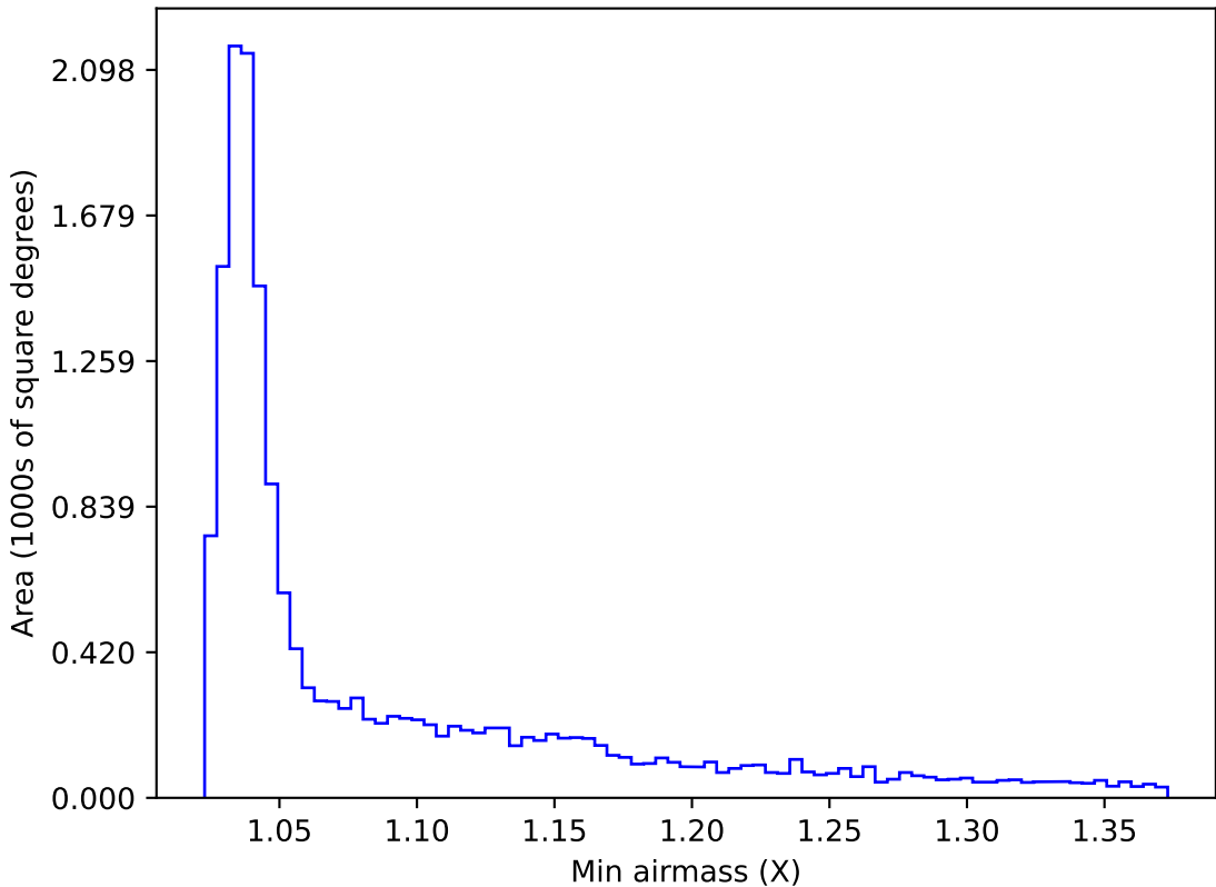
ddf_acor_sf15_lsf30_lsr20_v3.4_10yrs WFD g band: Min airmass
