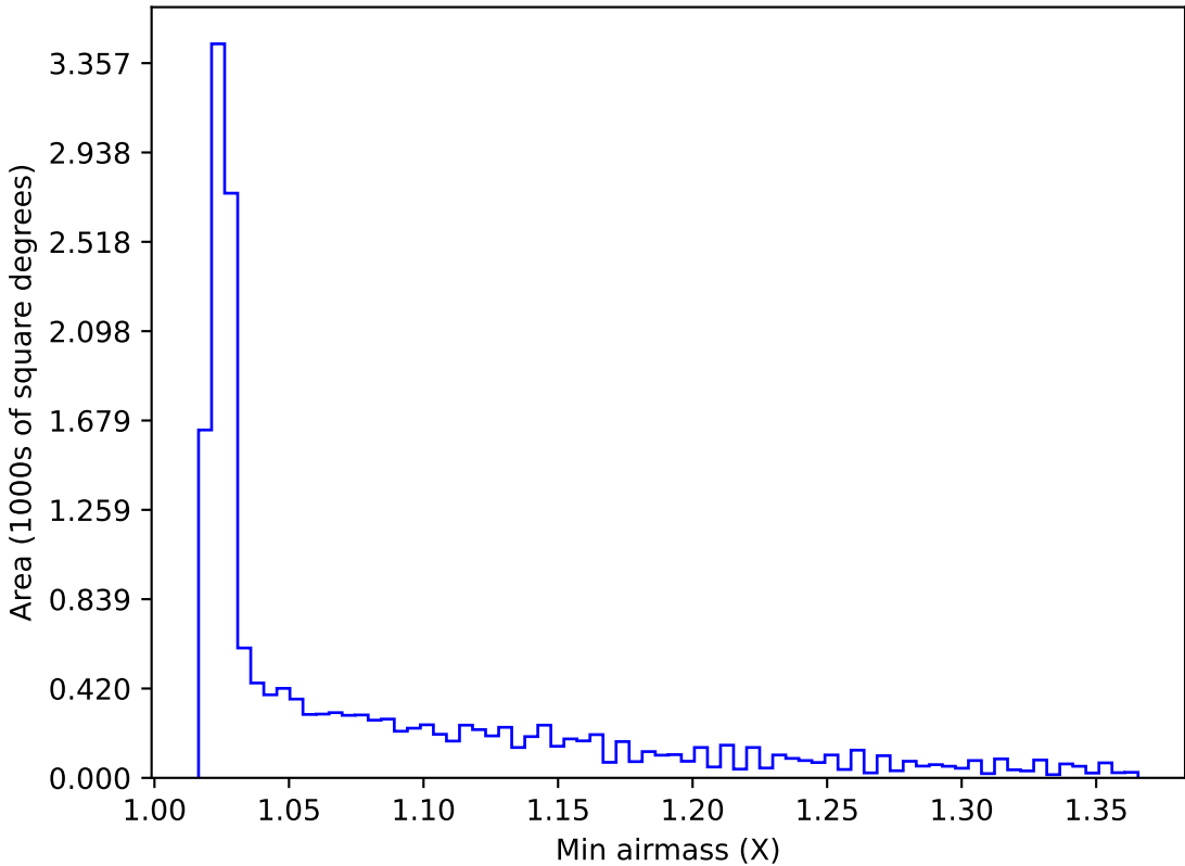
ddf_acor_sf15_lsf30_lsr20_v3.4_10yrs WFD all bands: Min airmass
