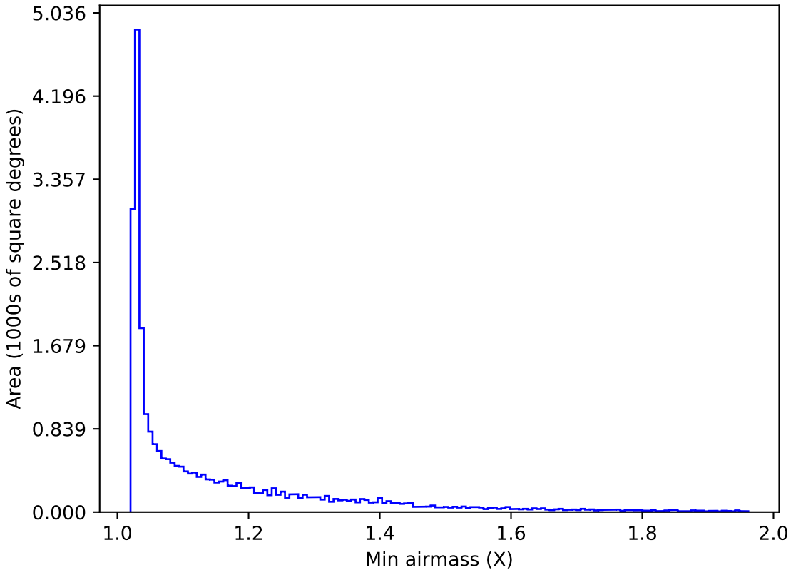
ddf_acor_sf15_lsf30_lsr20_v3.4_10yrs All sky z band: Min airmass
