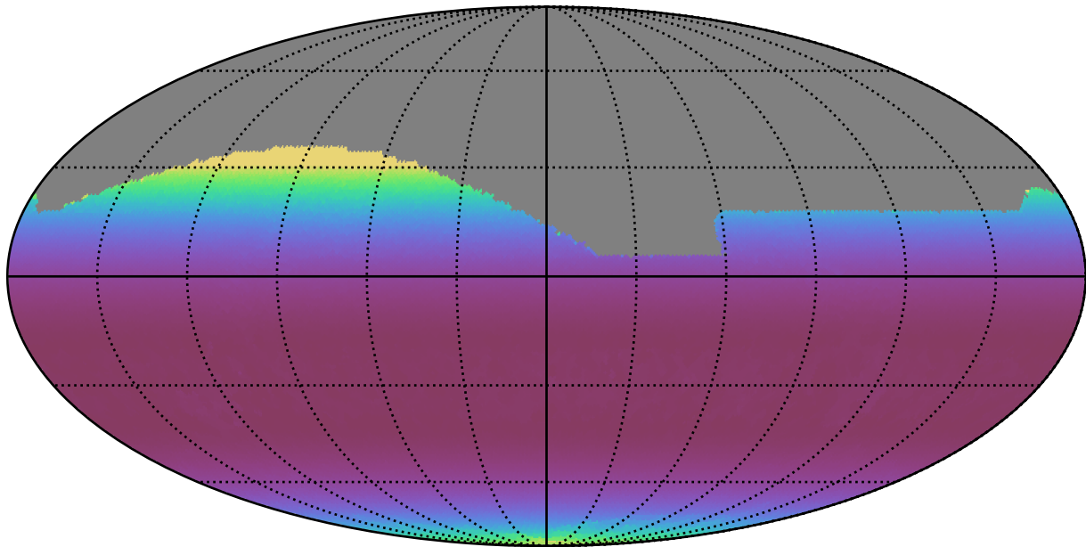
ddf_acor_sf15_lsf30_lsr20_v3.4_10yrs All sky r band: Min airmass
