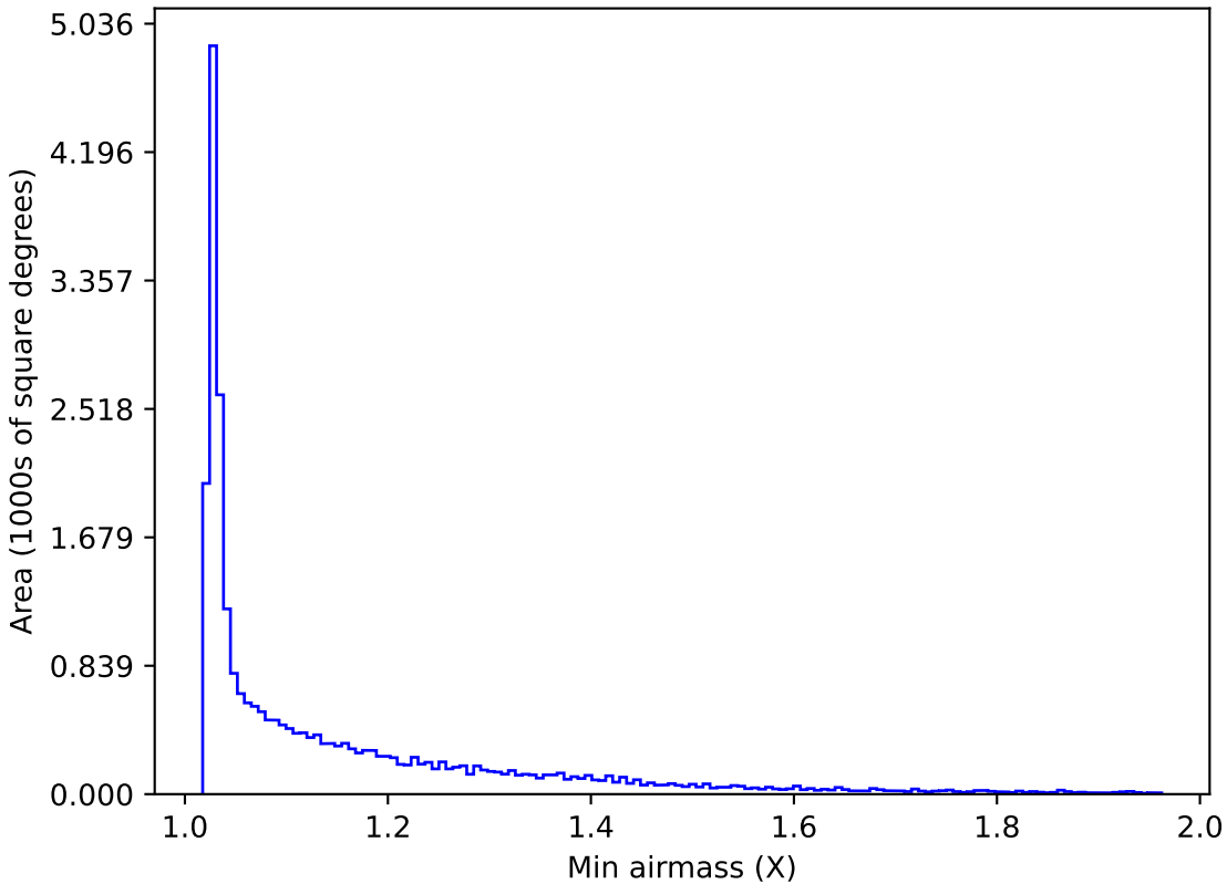
ddf_acor_sf15_lsf30_lsr20_v3.4_10yrs All sky r band: Min airmass
