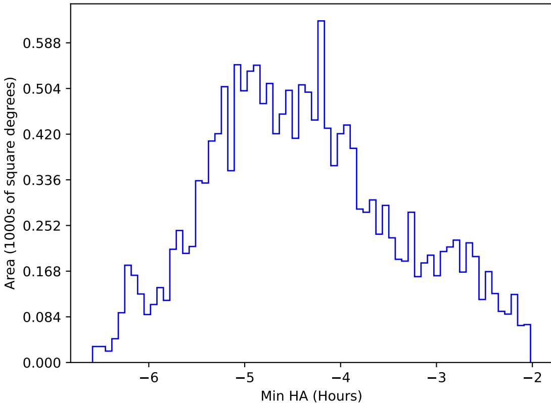
ddf_acor_sf15_lsf30_lsr20_v3.4_10yrs WFD z band: Min HA
