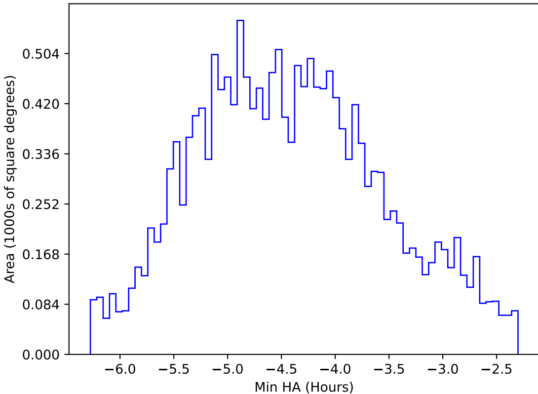
ddf_acor_sf15_lsf30_lsr20_v3.4_10yrs WFD r band: Min HA
