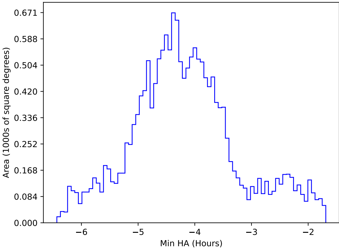
ddf_acor_sf15_lsf30_lsr20_v3.4_10yrs WFD g band: Min HA
