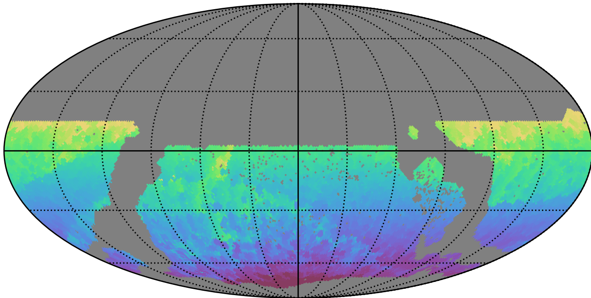
ddf_acor_sf15_lsf30_lsr20_v3.4_10yrs WFD all bands: Min HA
