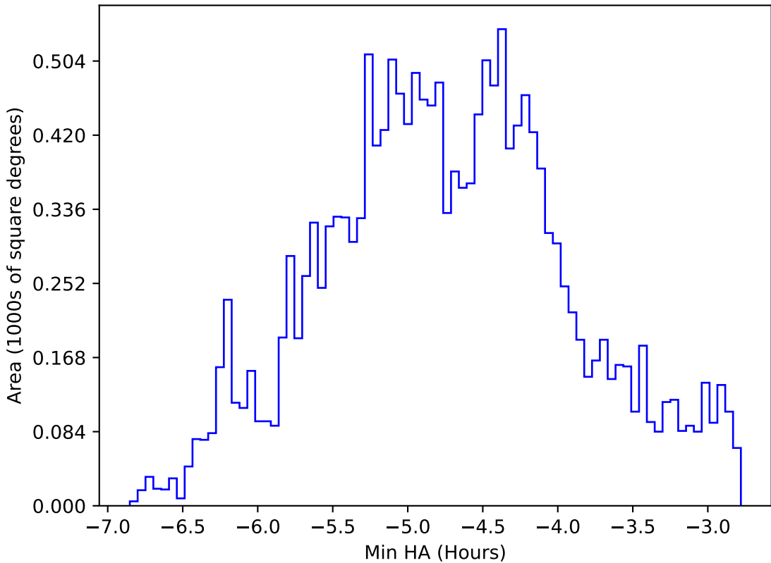
ddf_acor_sf15_lsf30_lsr20_v3.4_10yrs WFD all bands: Min HA
