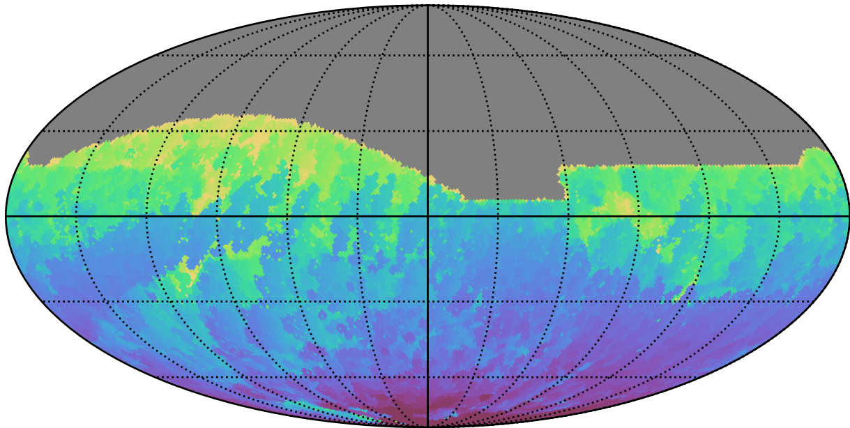
ddf_acor_sf15_lsf30_lsr20_v3.4_10yrs All sky z band: Min HA
