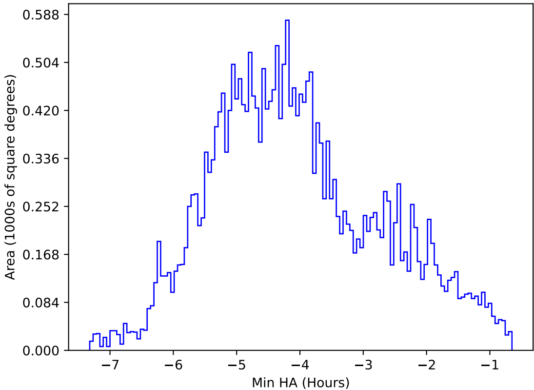
ddf_acor_sf15_lsf30_lsr20_v3.4_10yrs All sky z band: Min HA
