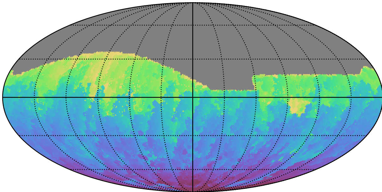
ddf_acor_sf15_lsf30_lsr20_v3.4_10yrs All sky g band: Min HA
