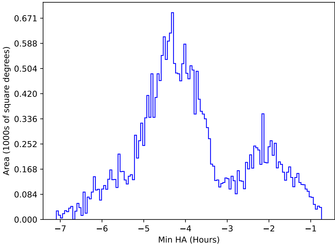
ddf_acor_sf15_lsf30_lsr20_v3.4_10yrs All sky g band: Min HA
